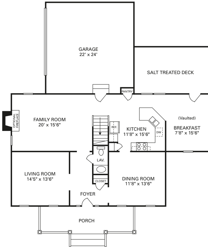
1st Floor
